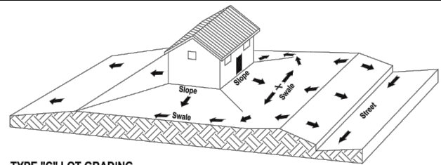
TYPE "C" LOT GRADING
