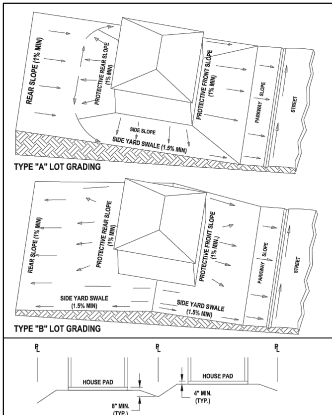
SIDEYARD SWALE (TYPICAL)
