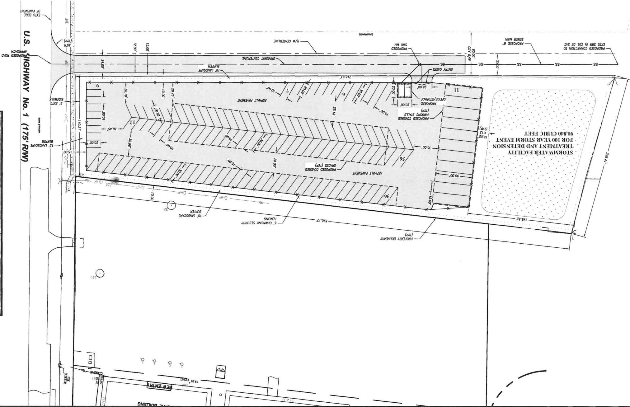
SITE PLAN 1" = 40'
