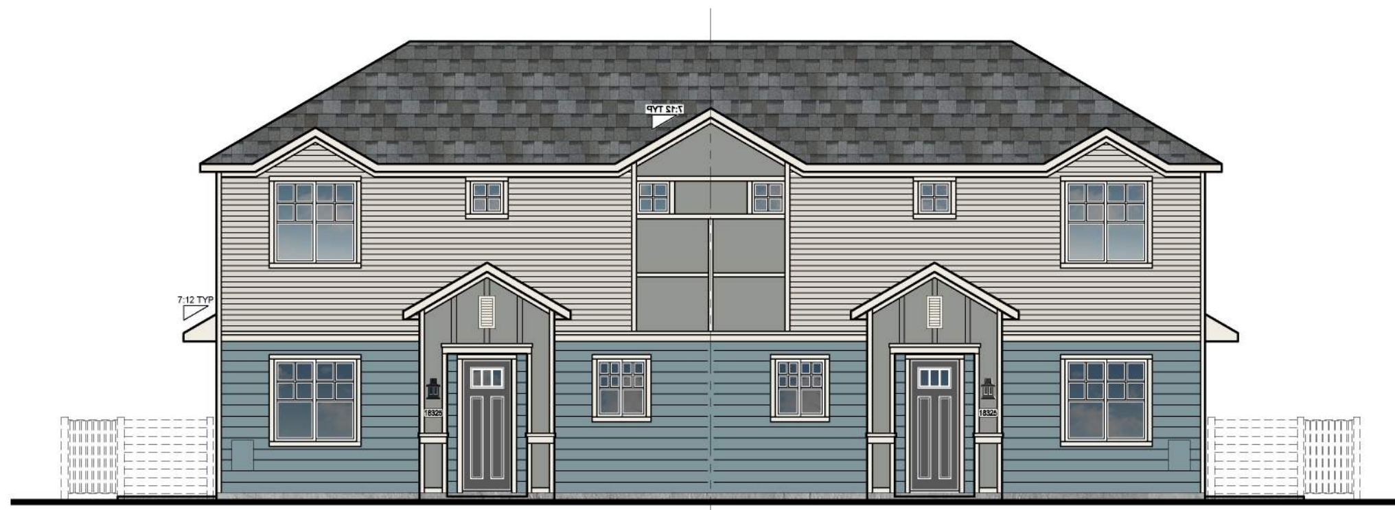
REAR ELEVATION COASTAL STYLE 1/8" = 1'-0"
