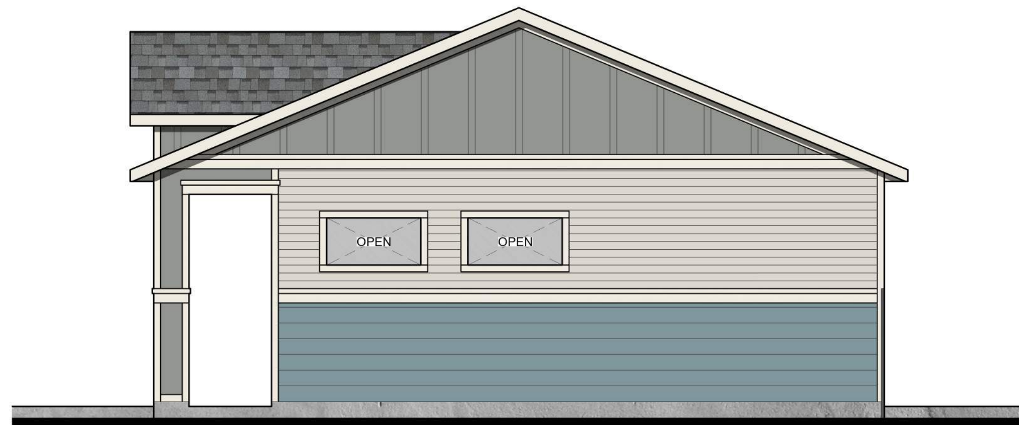
RIGHT ELEVATION COASTAL 1/4" = 1'-0"
